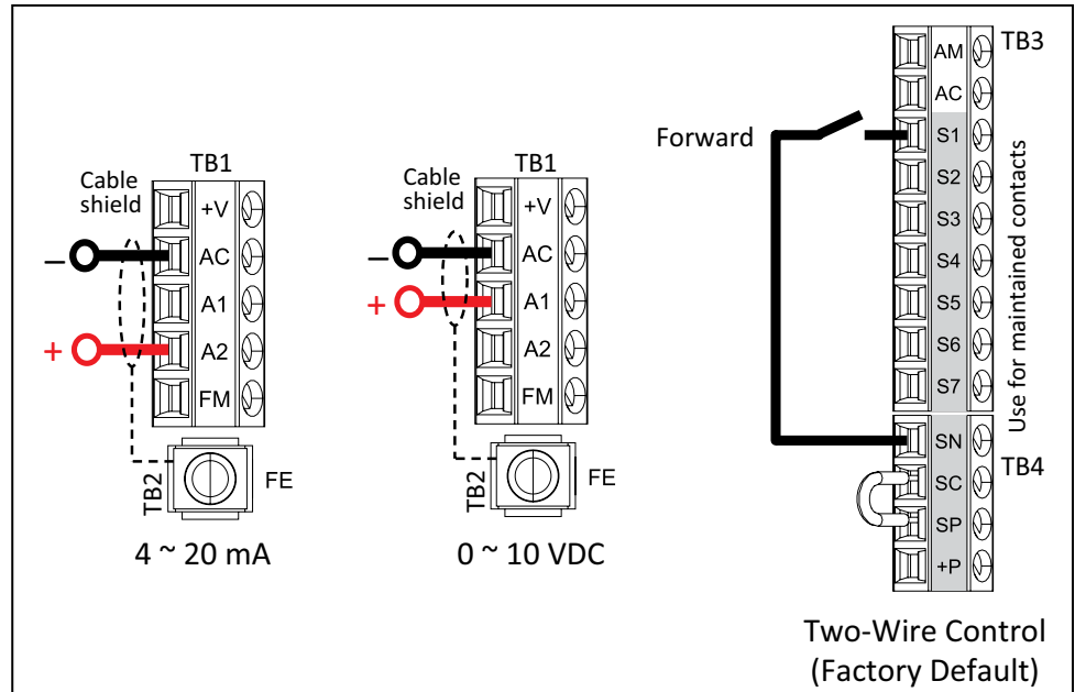
WIRING DETAILS
