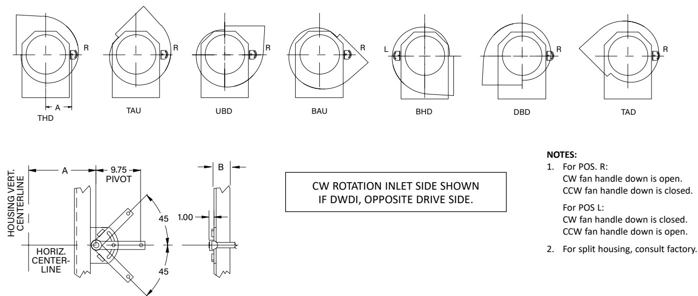
Figure 5. Nested Inlet Vane Handle Location For Rotatable Fans
