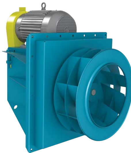
BEPL Arrangement 9 - Pedestal Plug Fan
