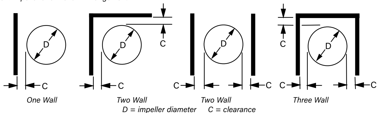
Figure 1. Impeller and Plenum Arrangement
