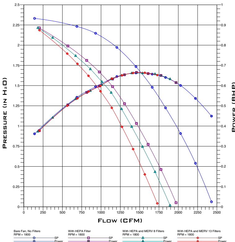
MODEL DSI, SIZE 140X PERFORMANCE CURVE
