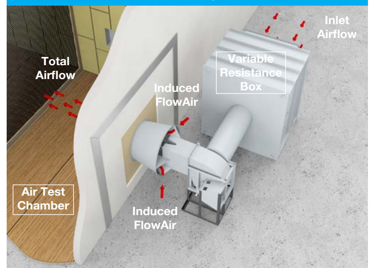
AMCA 260 - Figure 1
