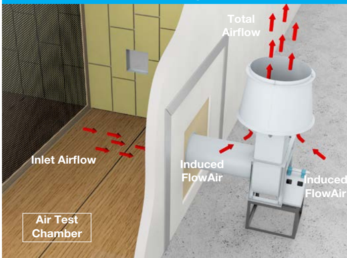
AMCA 210 - Figure 15
