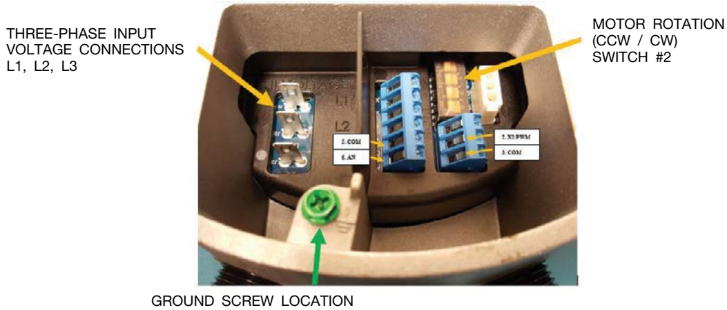
Figure 7. Connections for signal and power leads
